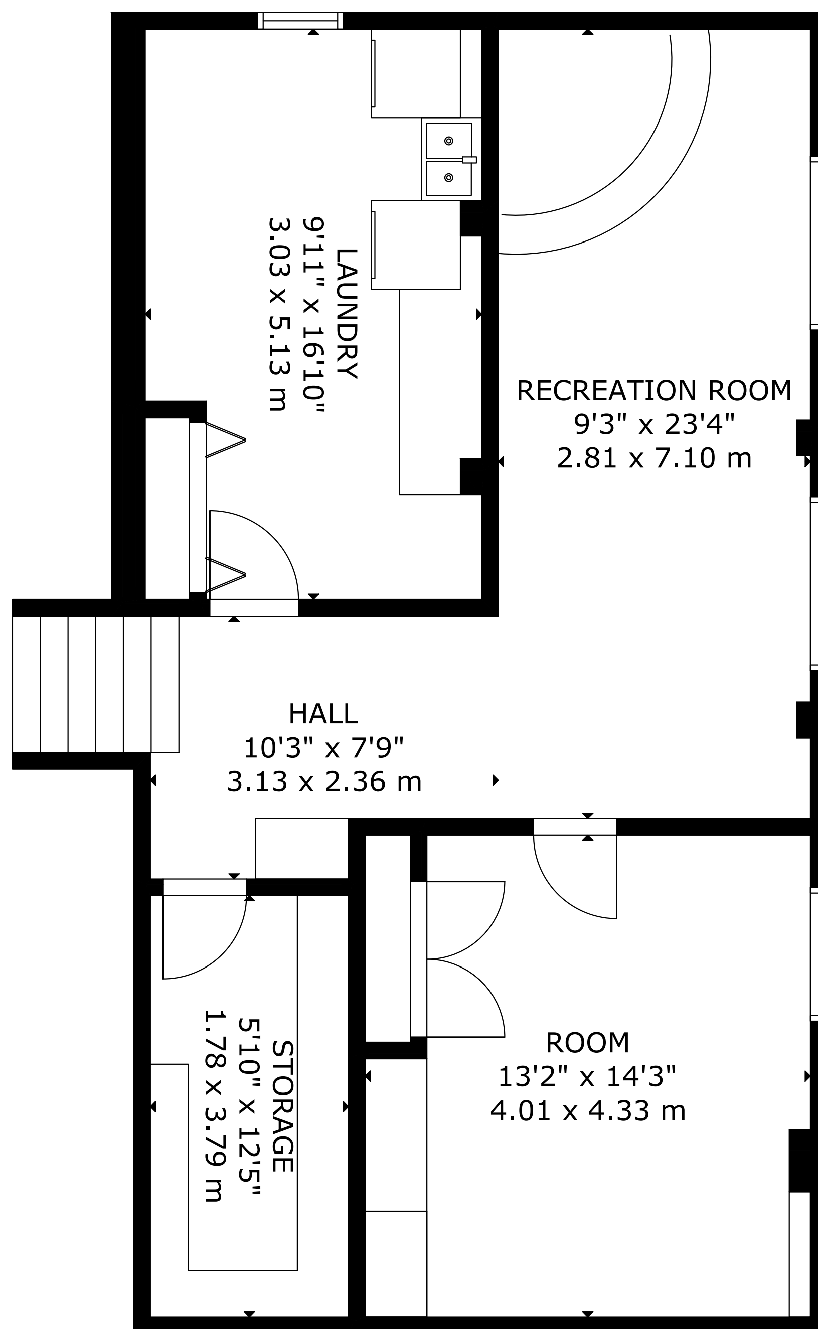
BASEMENT
