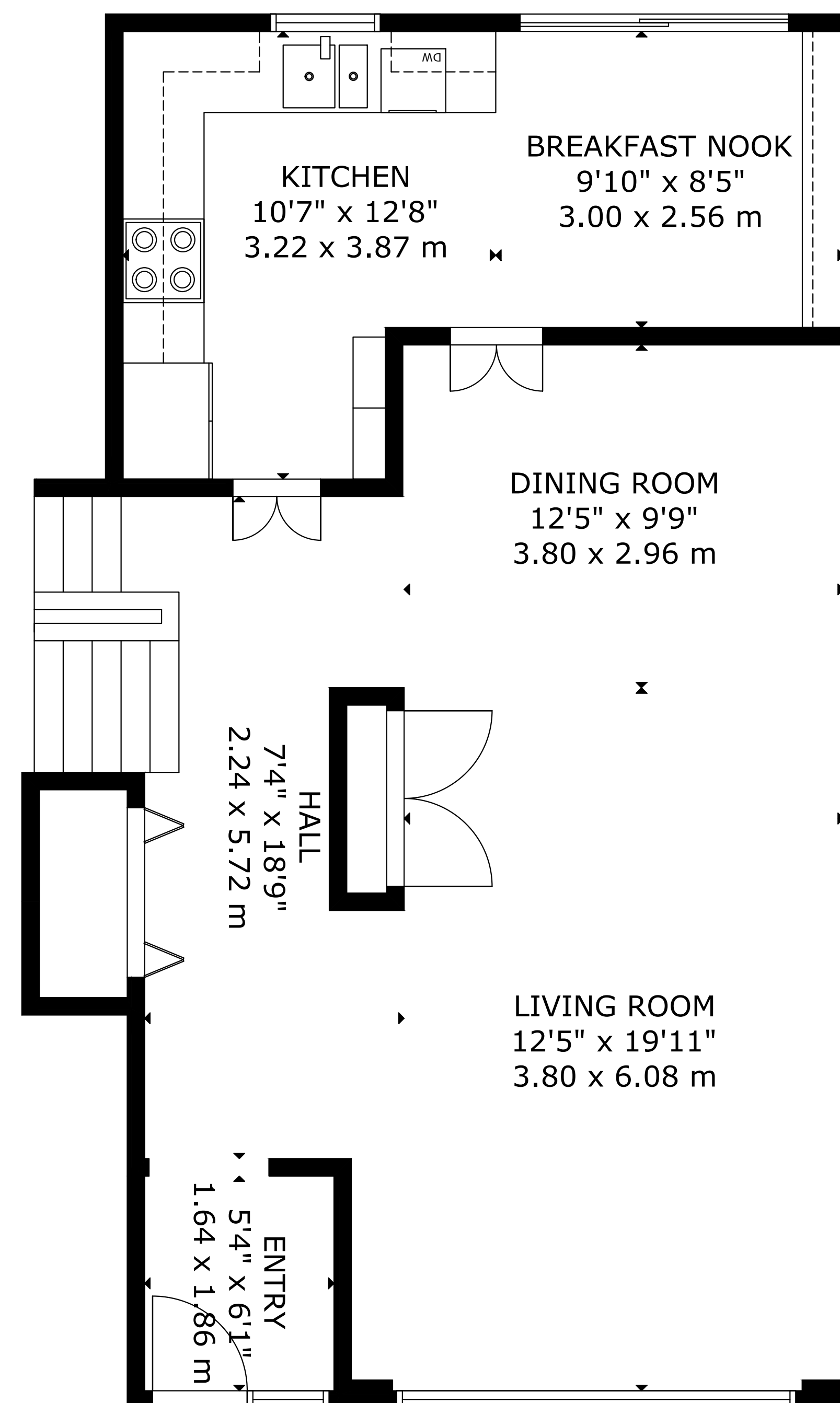
FIRST FLOOR
